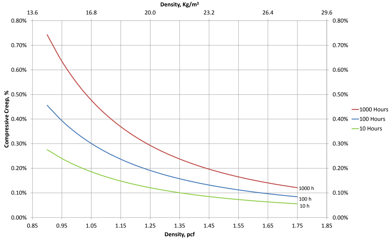
Density vs. Compressive Creep
